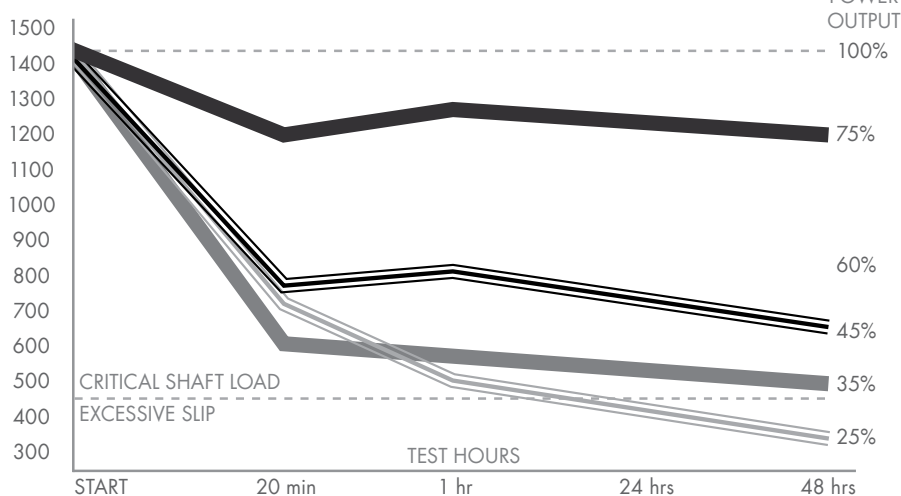
GRAPH : SHAFT LOAD LOSS WITH WEDGE BELT SPB 2000
